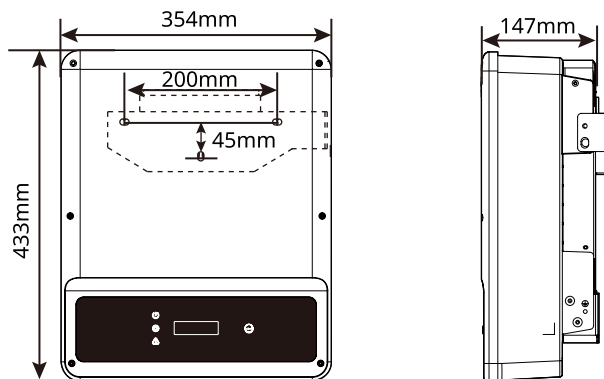
GW4K-DT, GW4000-SDT-20, GW5K-DT, GW5000-SDT-20, GW6K-DT, GW6000- SDT-20, GW8K-DT, GW10KT-DT
