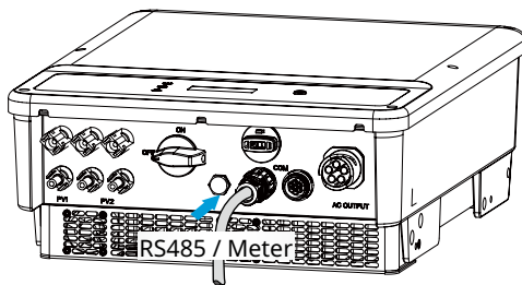
GW8K-DT, GW10KT-DT
