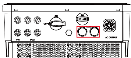
GW12KT-DT, GW15KT-DT
