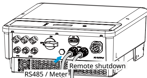
GW8K-DT, GW10KT-DT
