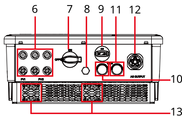
GW12KT-DT, GW15KT-DT
