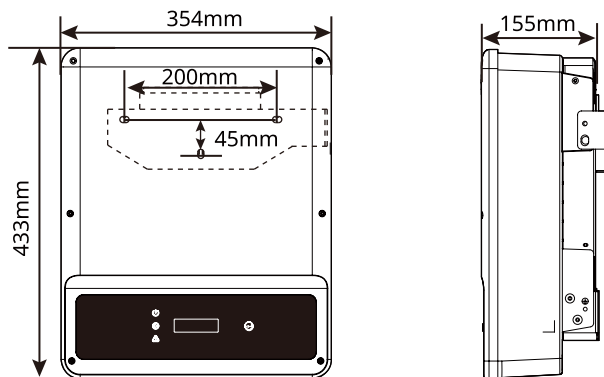
GW12KT-DT, GW15KT-DT
